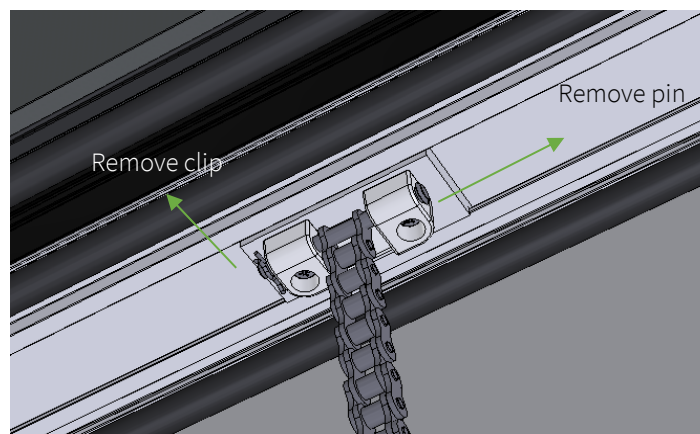
Figure 6 – Manual disconnect
