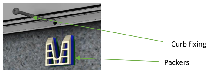
Figure 7 - Curb fixings
