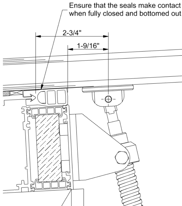
Figure 6 – Positioning of the lid bracket
