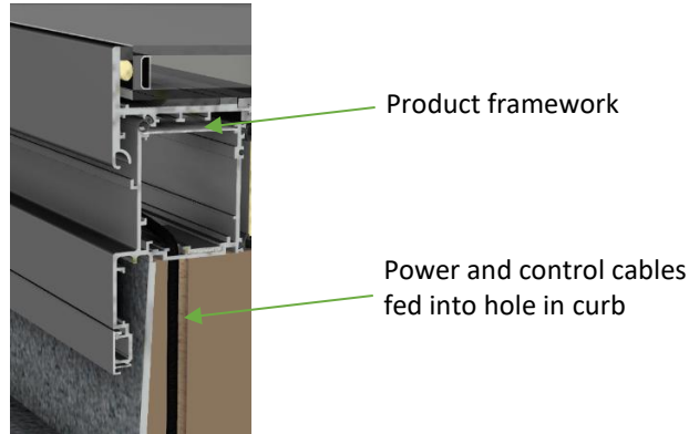
Figure 6 - Position of power and control cables in motor housing
