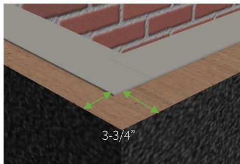
Figure 2 – Curb top trim measurements
