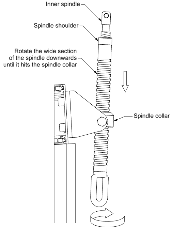
Figure 5 – Attach the spindle to the base bracket
