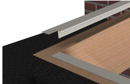
Figure 1 – Curb top trim placement
