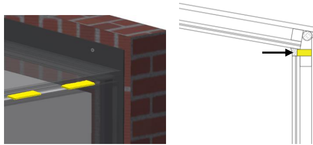
Figure 6 – Plastic packers used to support glass at joint
