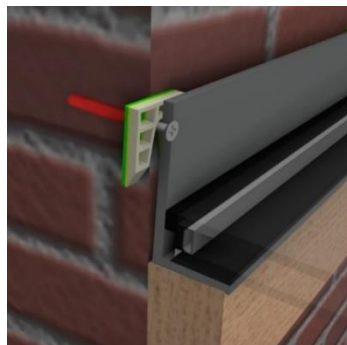
Figure 5 – Wall abutment fixed in place
