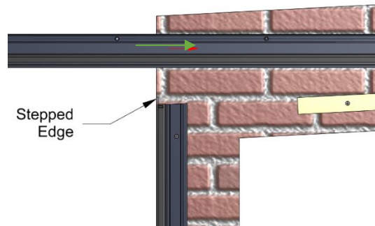
Figure 3 - Sliding the horizontal section into position
