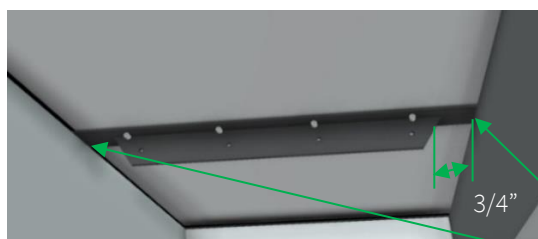
Figure 12 – Back-to-back angles
