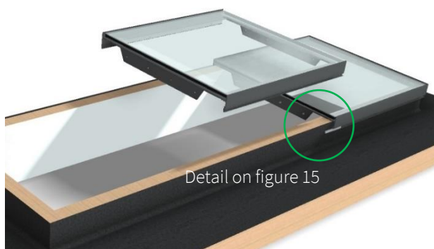
Figure 14 – Joining plate inserted
