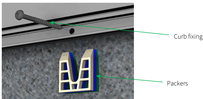
Figure 17 - Curb fixings
