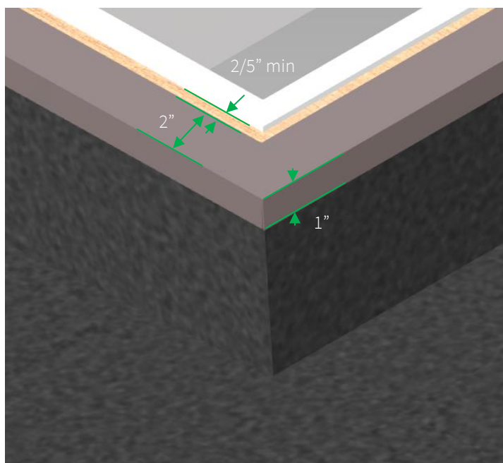
Figure 9 – Flashing Tape
