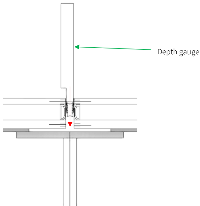
Figure 20 – Secondary Seal
