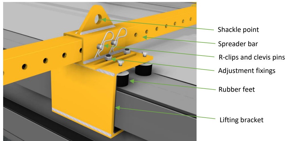
Figure 4 - Lifting bracket
