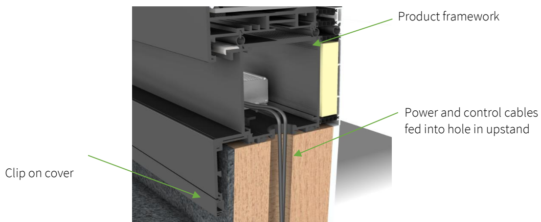
Figure 9 - Position of power and control cables in motor housing
