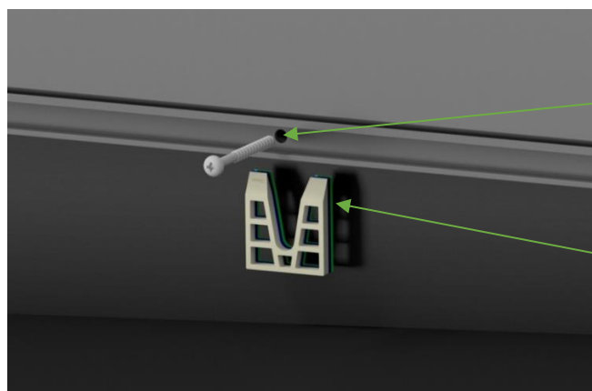
Figure 10 - Upstand fixings
