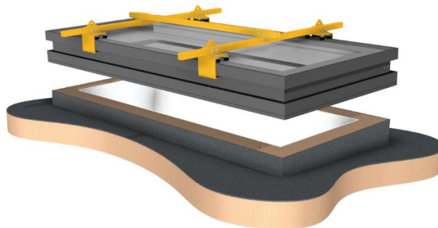
Figure 8 – Suggested lifting configuration
