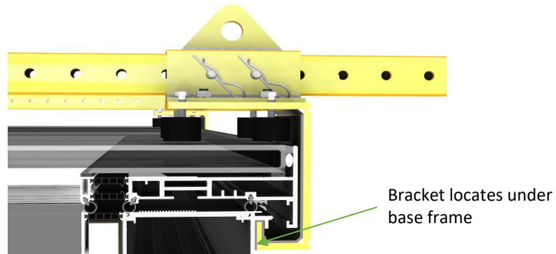
Figure 5 - Locating position
