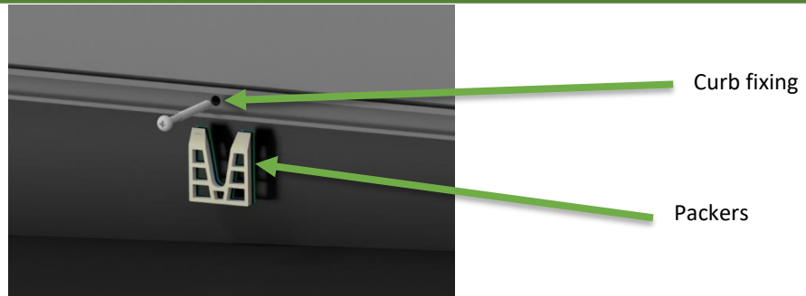
Figure 10 - Curb fixings
