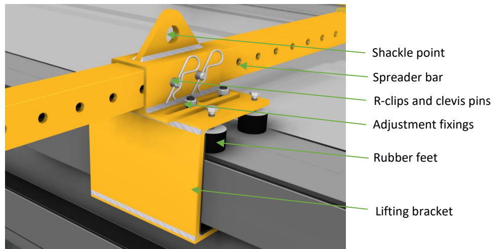
Figure 4 - Lifting bracket
