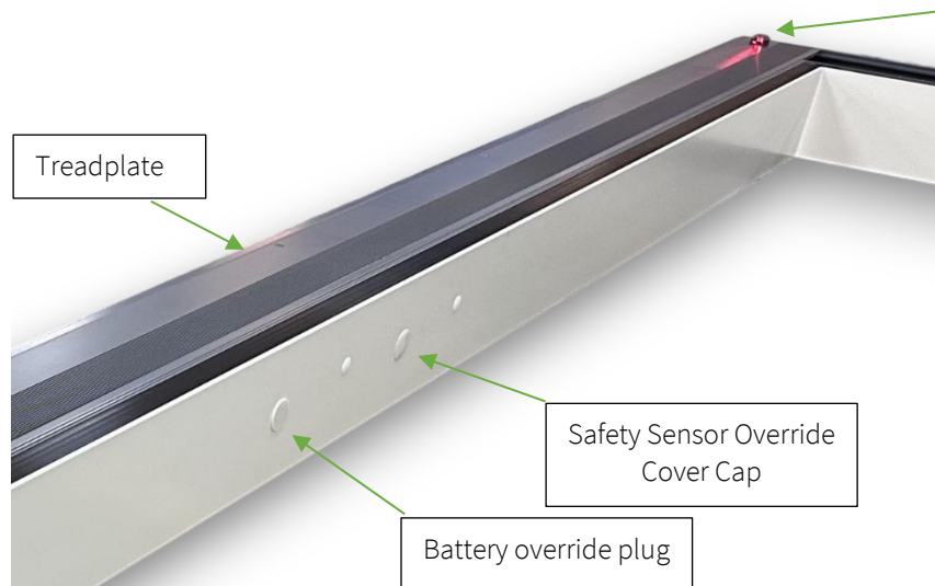
Figure 10 – Safety sensor override
