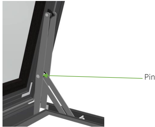
Figure 8 – Mechanism disassembly
