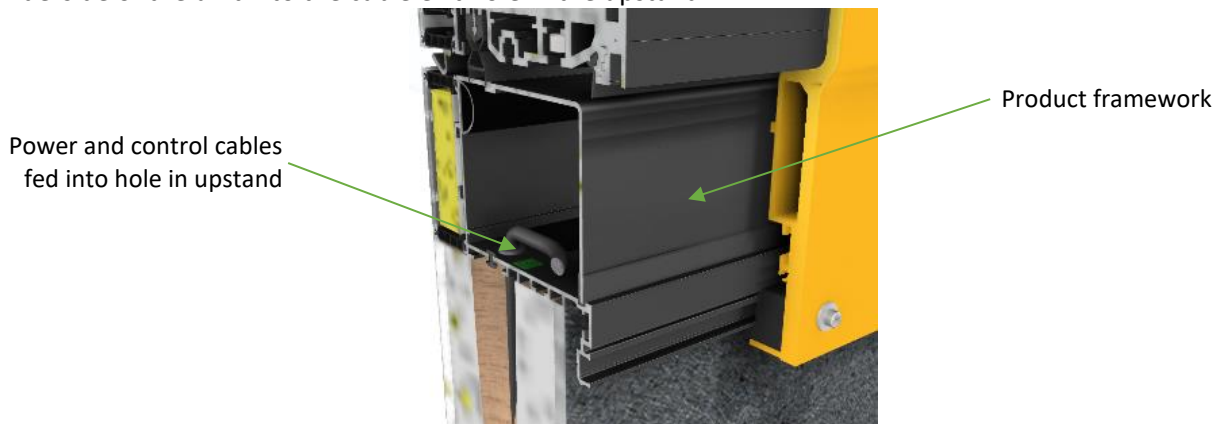
Figure 10 - Position of power and control cables in motor housing
