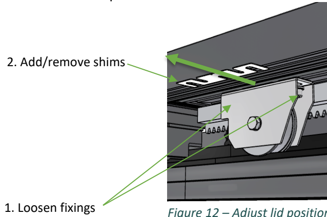
Figure 12 – Adjust lid position
