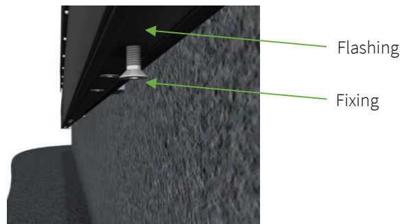
Figure 13 – Flashing fixings
