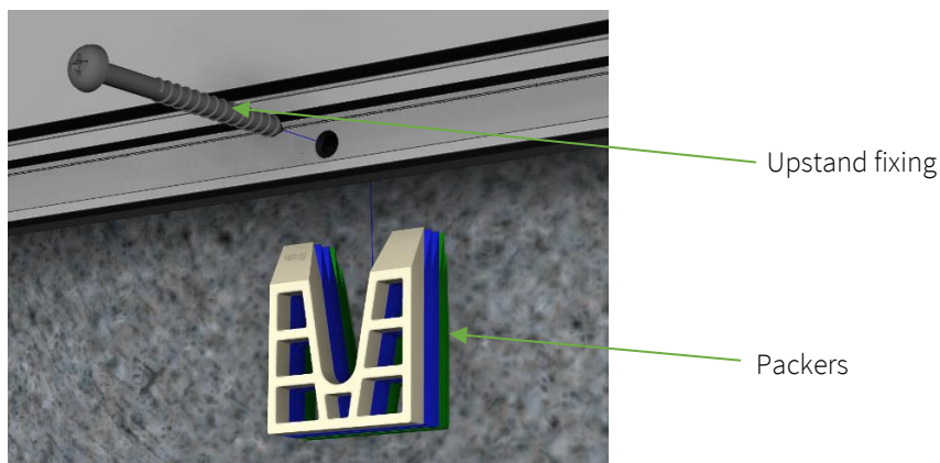
Figure 11 - Upstand fixings
