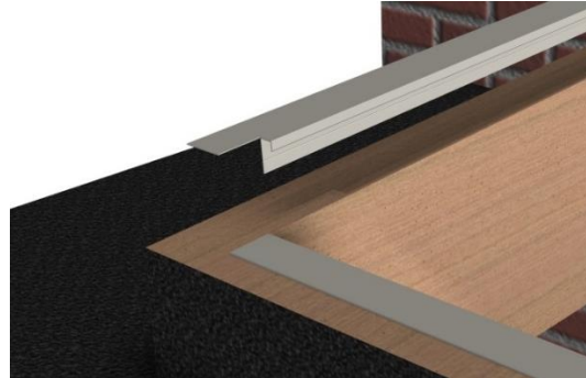
Figure 1 – Upstand top trim placement
