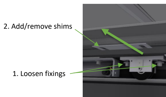
Figure 9 – Adjust door position
