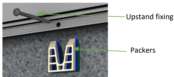
Figure 8 - Upstand fixings
