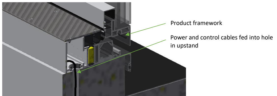
Figure 7 - Position of power and control cables in motor housing
