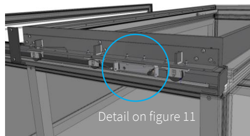
Figure 10 – View of the override mechanism
